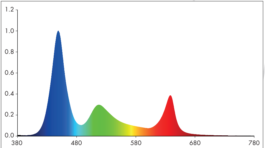
Full RGBW (wide beam) : Flux=7100 lm
